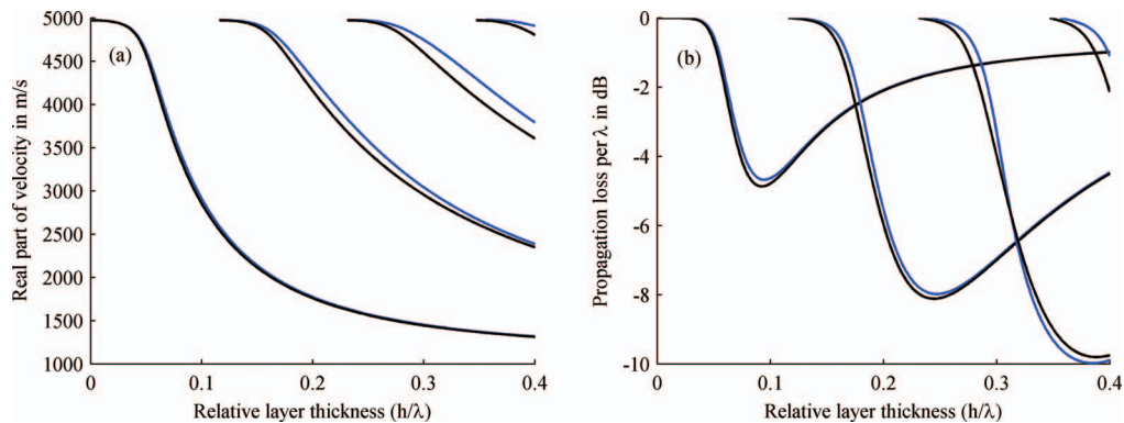
FIG. 5. The real part of velocity and propagation loss vs. relative layer thickness for a LW device with a viscoelastic guiding layer. (a) real part of velocity; (b) propagation loss. The black lines in (b) denote the propagation loss scaled up by a factor of 1000.
